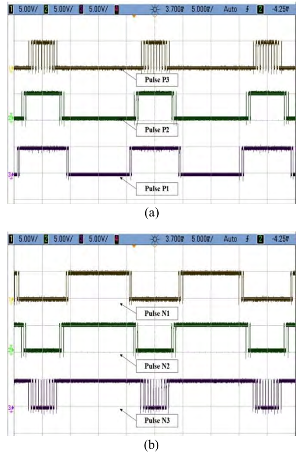
FIGURE 7. PWM pulse pattern for 5 switch module. (a) Positive half cycle (b) Negative half cycle.
