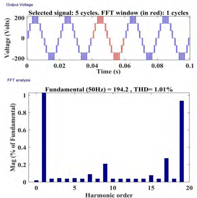
FIGURE 12. Output Voltage and FFT plot for 8 switch module.
