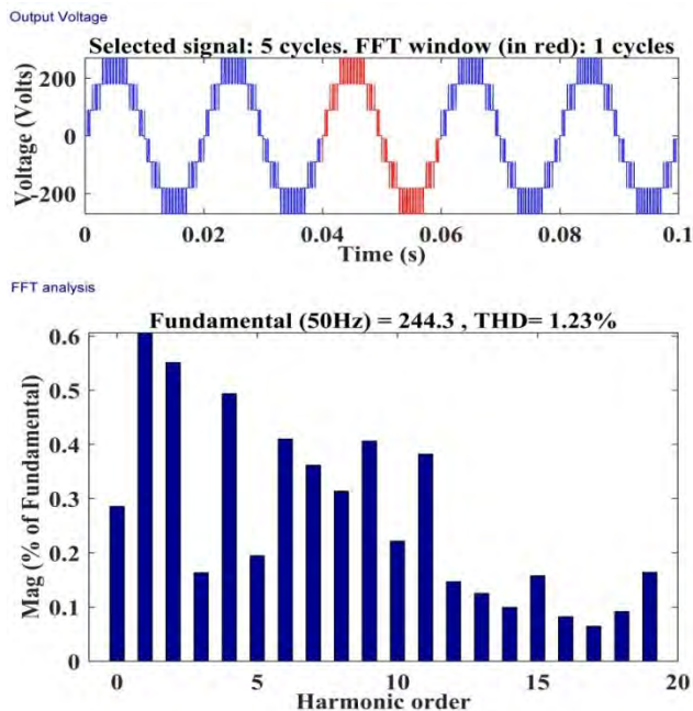
FIGURE 11. Output Voltage and FFT plot for 5 switch module.
