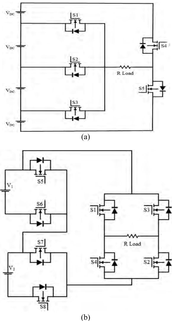
FIGURE 1. (a) Structure of 5 Switch MLI. (b) Structure of 8 Switch MLI.
